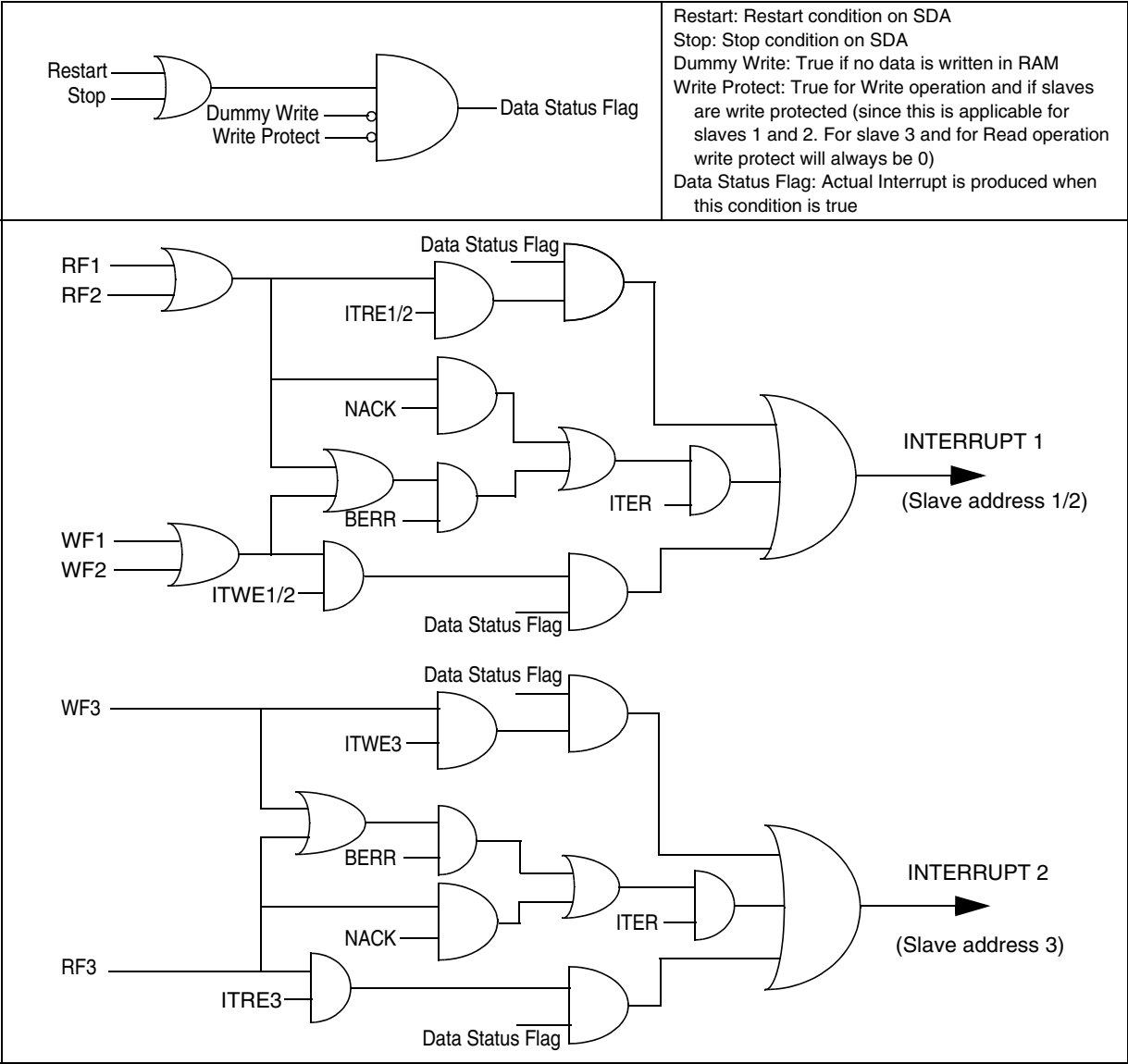
Figure 80. Event Flags and Interrupt Generation
