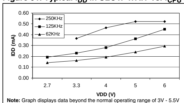
Figure 91. Typical I_{DD} in SLOW-WAIT vs. f_{CPU}
