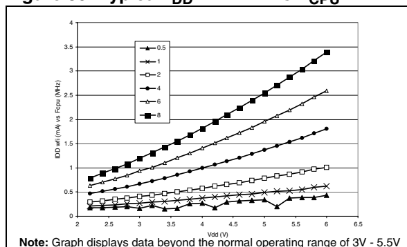
Figure 89. Typical I_{DD} in WAIT vs. f_{CPU}
