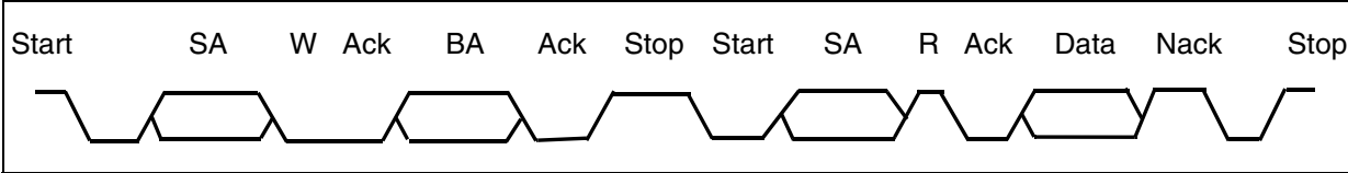
Figure 78. Sequential Read
