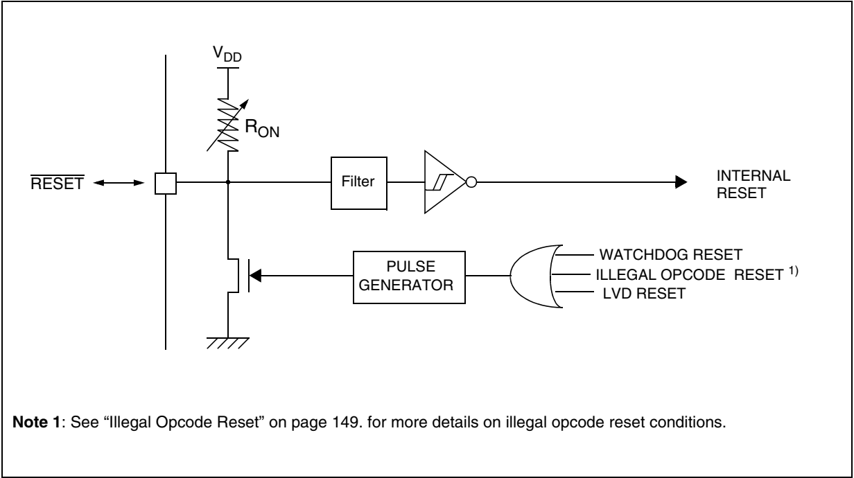
Figure 16. Reset Block Diagram
